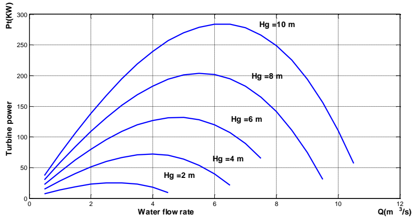
Fig. 4. Variation of turbine power with water flow rate at different values of gross head.
