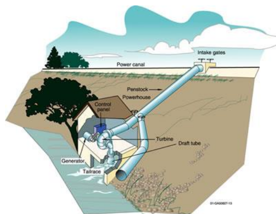
Fig. 1. Schematic diagram of micro-hydro-electric power plant.
