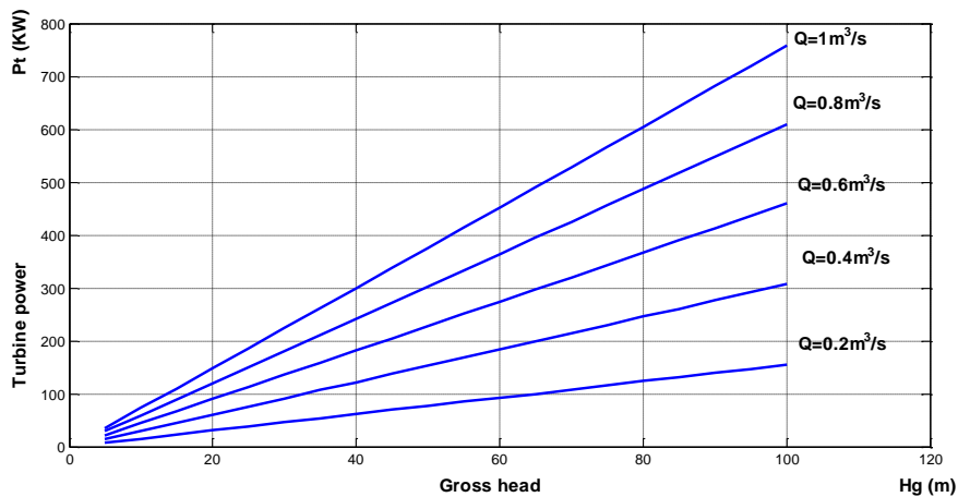
Fig. 2. Variation of turbine power with gross head at different values of water flow rate.
