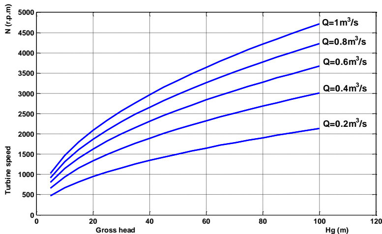
Fig. 3. Variation of turbine speed with gross head at different values of water flow rate.
