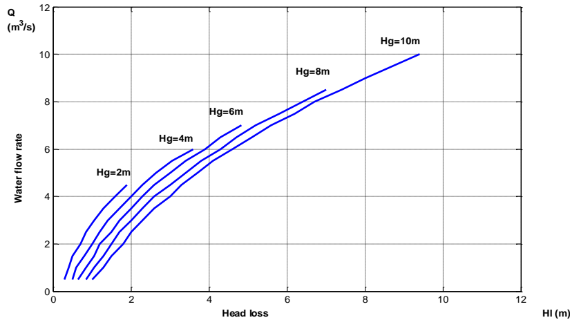
Fig. 7. Variation of water flow rate with head loss at different values of gross head.
