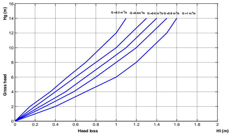
Fig. 6. Variation of gross head with head loss at different values of water flow rate.
