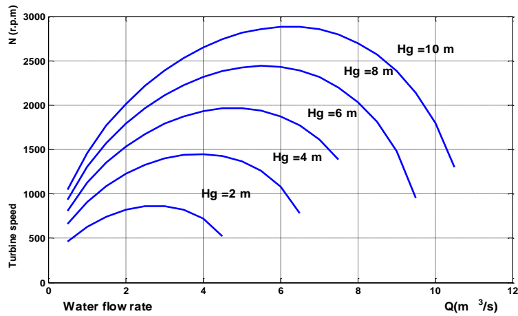
Fig. 5. Variation of turbine speed with water flow rate at different values of gross head.
